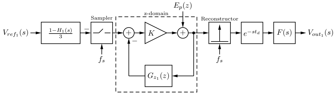
Figure 6.5: Inner loop with sampling comparator model.
