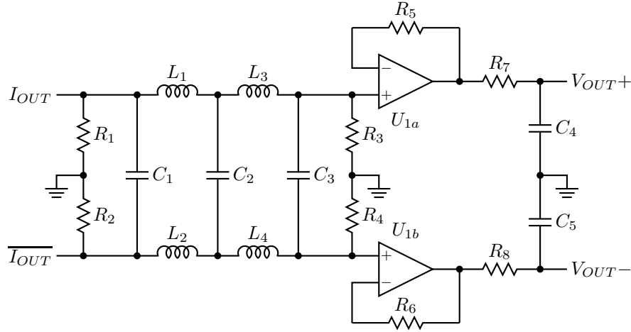
Figure 4.2: DAC output filter and buffer.
