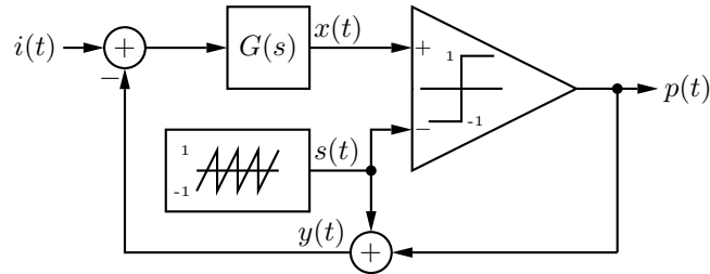
Figure 2.10: Simple PWM feedback loop with ripple compensation [2].
