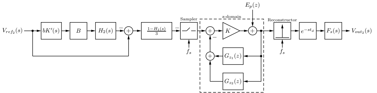
Figure 6.7: Complete loop with sampling comparator model.
