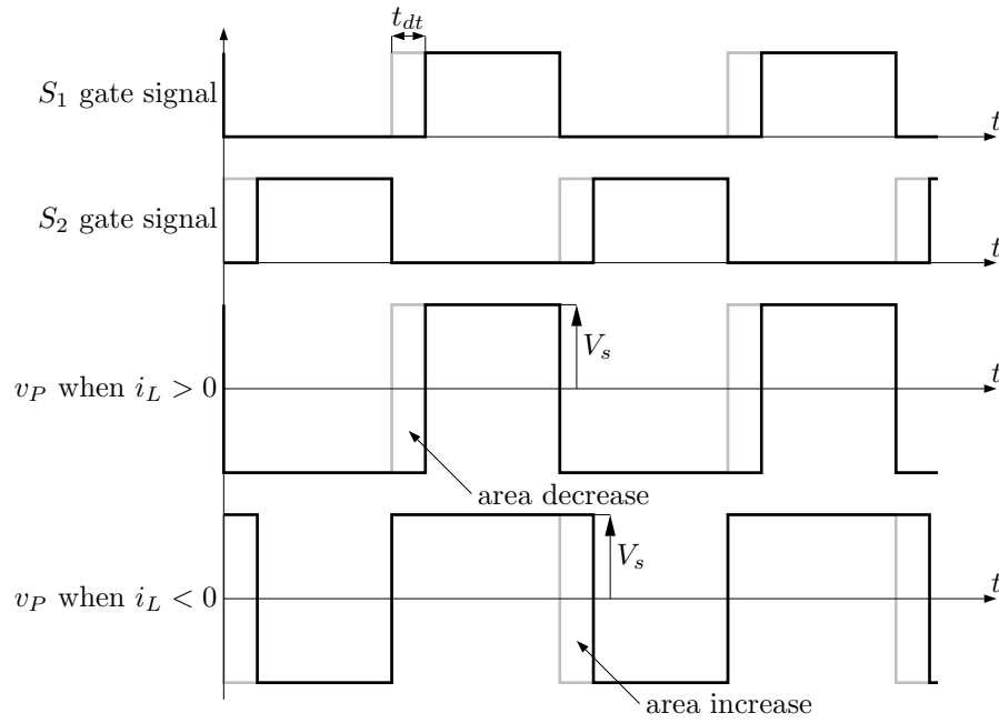
Figure 2.3: The effect of dead time on converter waveforms. Ideal waveforms are shown in grey.
