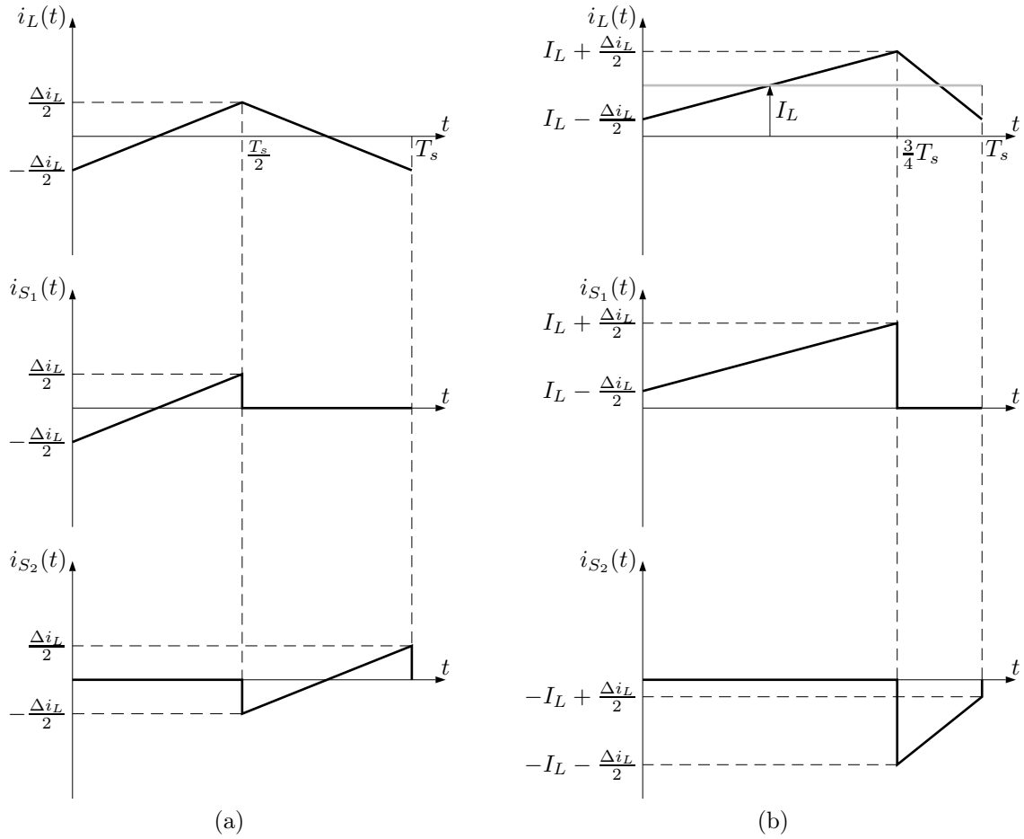
Figure 2.5: Idealised inductor and supply current waveforms for (a) D = 0.5 and (b) D = 0.75 .
