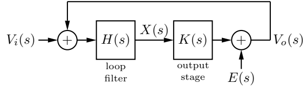
Figure 2.13: Generic output stage embedded in a feedback loop.
