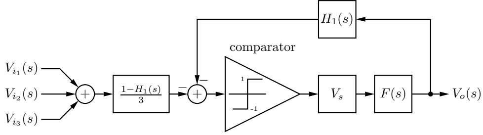
Figure 5.4: Control system block-diagram of output stage with passive compensation.
