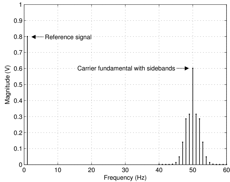
Figure 2.1: Calculated magnitude spectrum of ideal NSSSPWM for m_a = 0.8 and m_f = 50 .
