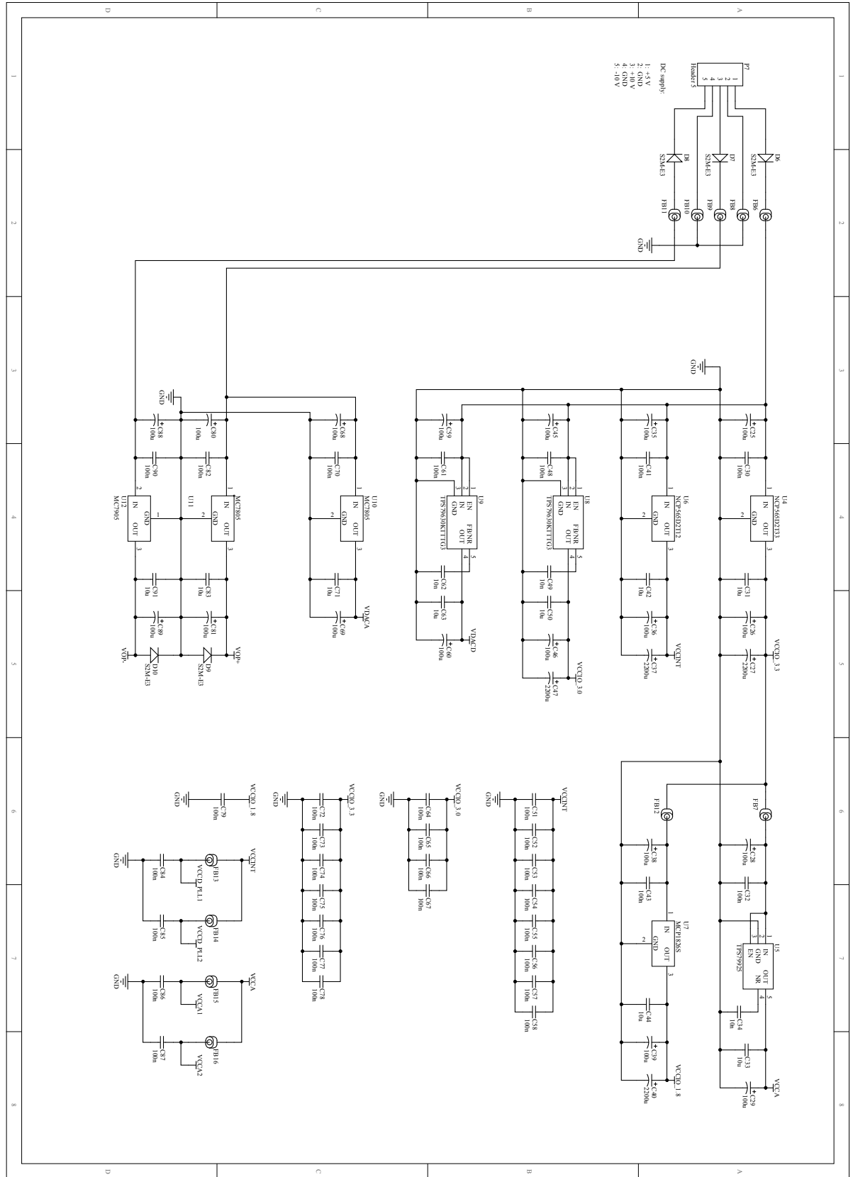
Figure A.4: FPGA carrier generator schematic (part one).
