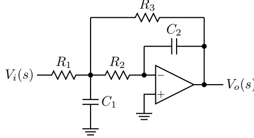
Figure 7.6: Estimation filter stage circuit.
