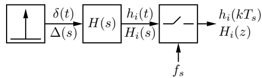
Figure 6.1: Block diagram illustration of the impulse invariant method.
