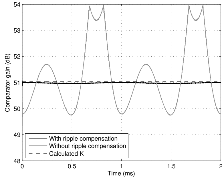
Figure 8.3: Simulated comparator gain with and without ripple compensation. The input signal frequency is 1 kHz and m_a = 0.8 .
