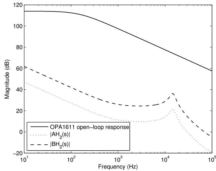
Figure 7.16: Open-loop frequency response of the OPA1611 op-amp, and transfer functions |AH_2(s)| and |BH_2(s)| .
