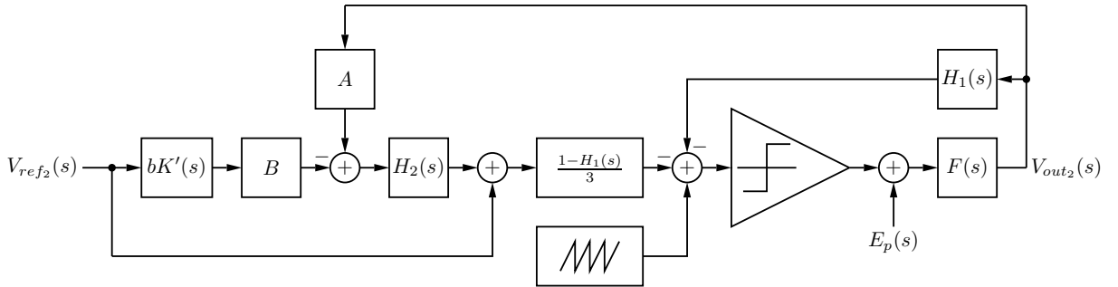
Figure 6.6: Continuous-time complete loop.
