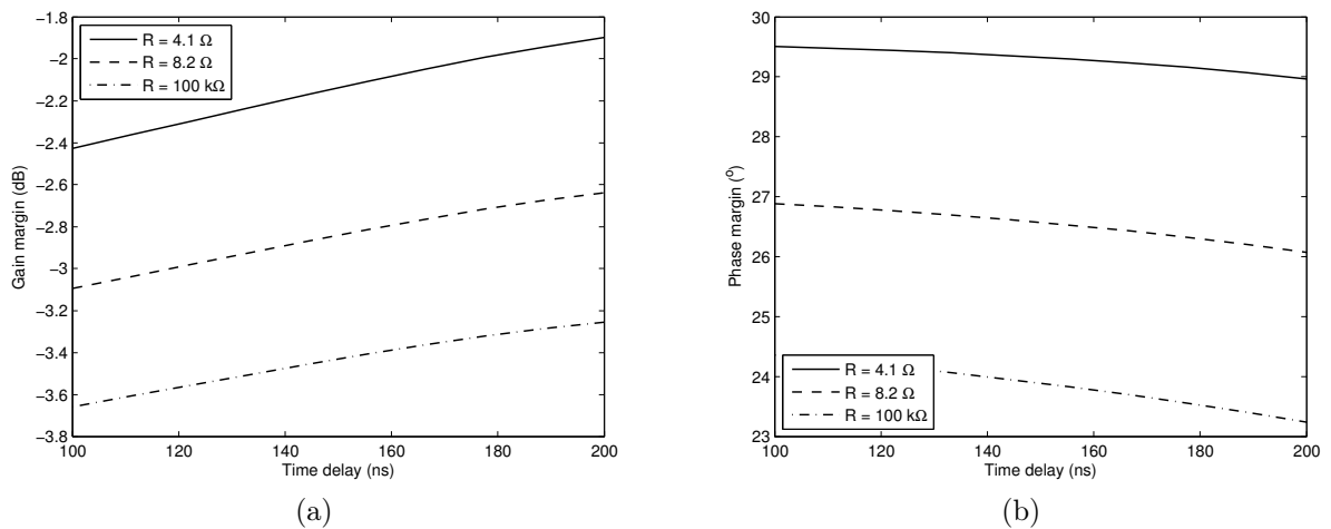
Figure 7.13: Gain margin (a), and phase margin (b), versus propagation delay for different loads.
