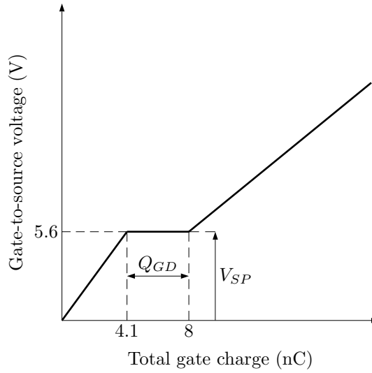
Figure 3.4: IRFI4019H-117P gate charge versus gate-to-source voltage [3].
