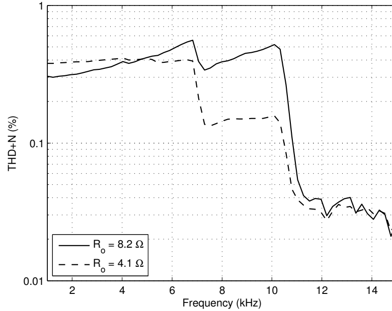
Figure 3.19: Open loop THD+N versus frequency for 10 W into 4.1 \Omega and 8.2 \Omega .
