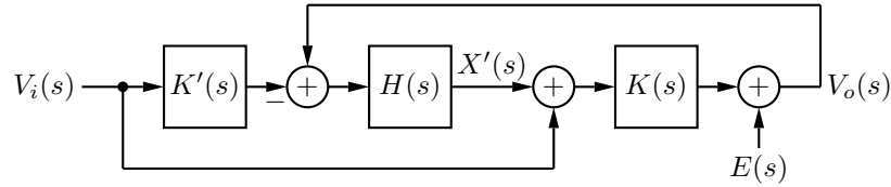
Figure 2.14: Modified control loop with deviation detection filter.
