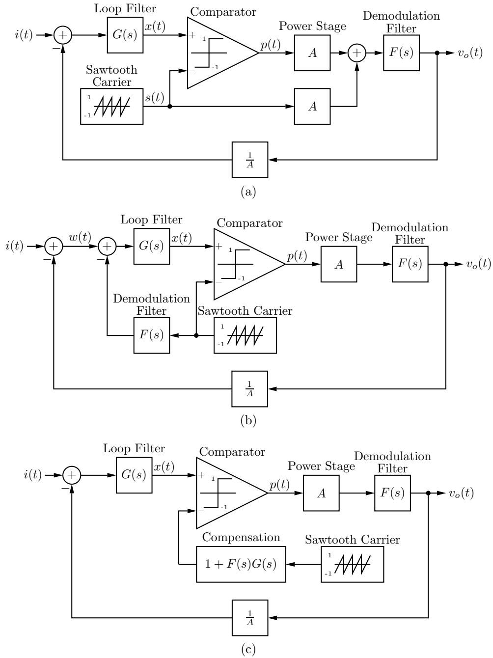
Figure 2.12: Three equivalent implementations of the ripple compensation technique obtained through block diagram manipulation [2].
