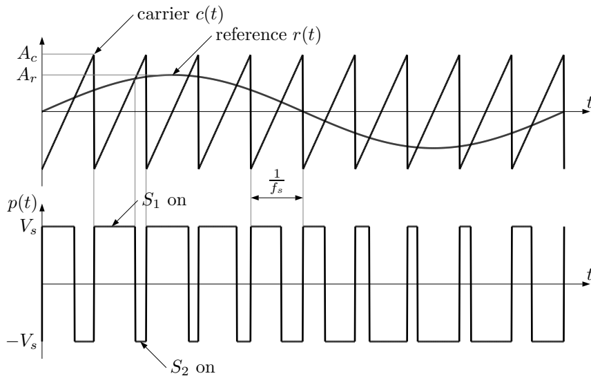
Figure 1.2: NSPWM waveforms for the converter of Figure 1.1.
