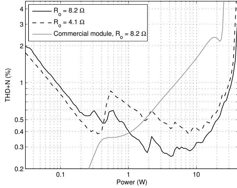
Figure 3.17: Open loop THD+N versus output power for R_o = 4.1 \Omega and R_o = 8.2 \Omega with a 1 kHz test signal.
