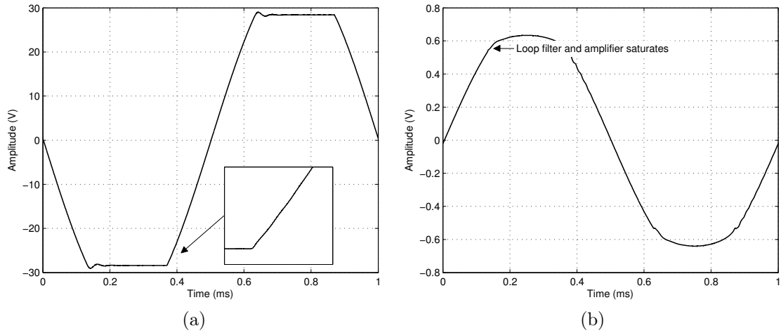
Figure 8.6: Spice simulation of amplifier output (a) and outer loop filter output (b) during over-modulation for R_2 = 3.25 \text{ k}\Omega .
