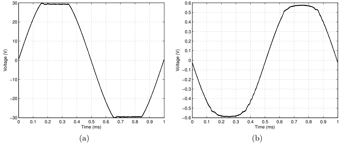
Figure 9.1: Oscilloscope measurements of (a) the output of the amplifier and (b) the output of the outer loop filter for m_a > 1 .
