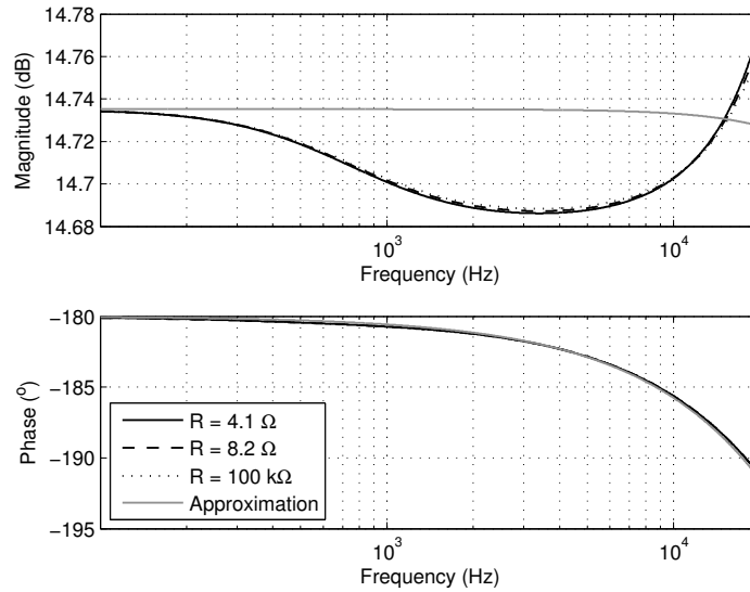
Figure 7.15: Calculated closed-loop transfer function STF_2(f) of the complete loop for output loads R = 4.1 \Omega , R = 8.2 \Omega and R = 100 \text{ k}\Omega . The grey line is an approximation.
