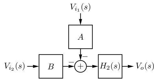
Figure 5.7: Control system block diagram of single op-amp third-order integrating loop filter.
