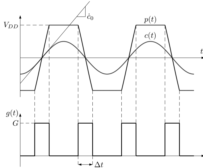
Figure 2.7: Comparator waveforms [1].
