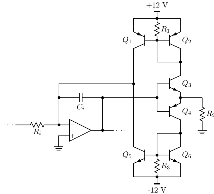
Figure 7.18: Transistor-based loop filter saturation circuit.
