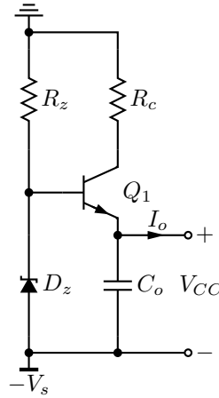
Figure 3.3: Low-side V_{CC} supply.
