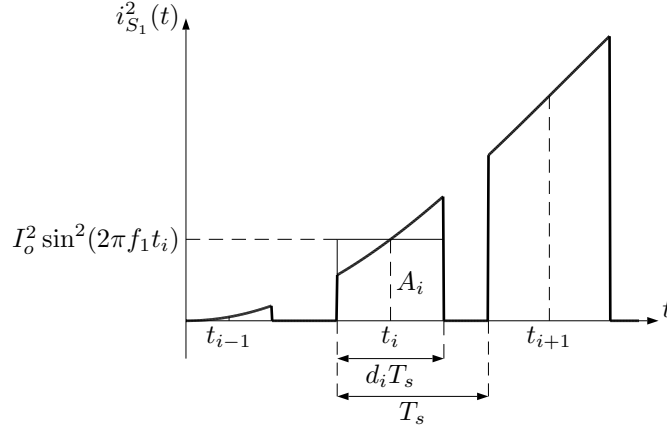
Figure 3.7: Square of the current through MOSFET S_1 with a sinusoidal current source as load. Three switching cycles are shown.
