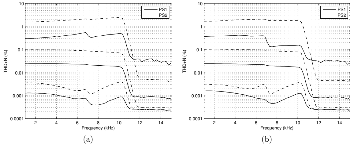
Figure 9.3: Measured THD+N versus frequency at 10 W with (a) R_o = 8.2\ \Omega and (b) R_o = 4.1\ \Omega . From top to bottom: open loop, with the inner control loop active, and with the complete control loop active.
