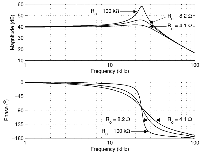
Figure 3.20: Measured open loop frequency response for various output loads. Bandwidth is >500\text{ kHz} .
