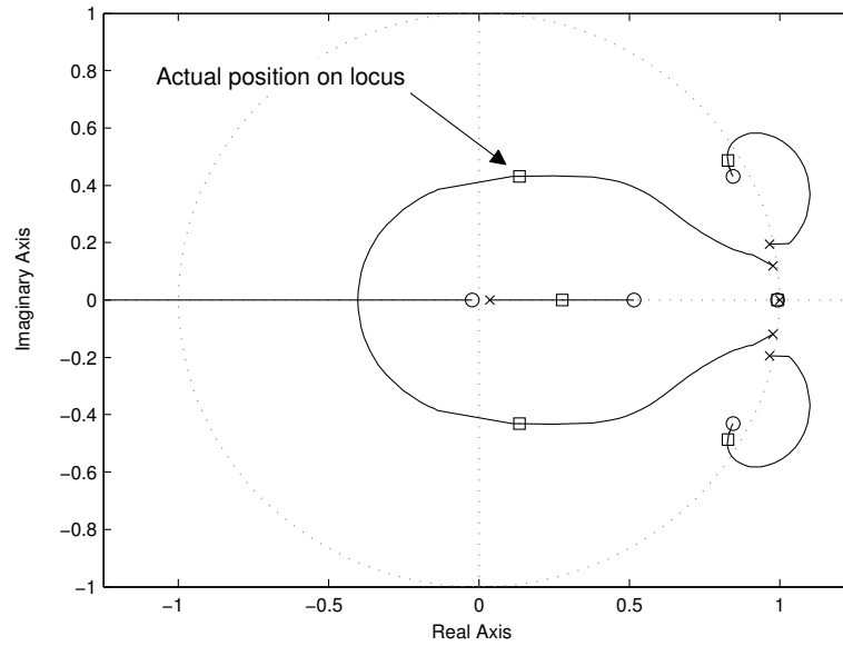
Figure 7.10: Root locus of complete control loop with an output load of R_o = 100 \text{ k}\Omega .
