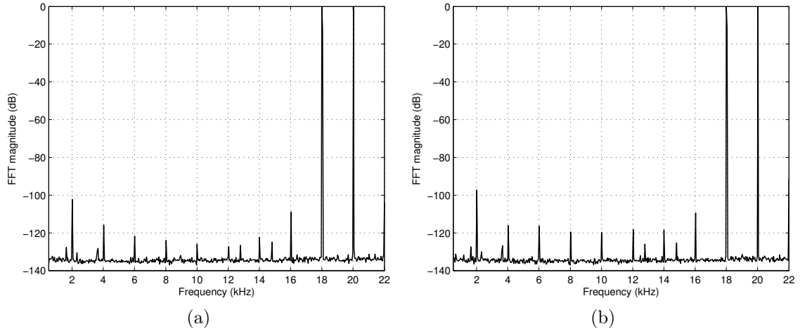
Figure 9.7: Normalised FFT of the amplifier output with 18 kHz and 20 kHz input tones for (a) PS1 and (b) PS2. Output power is 10 W into 8.2 \Omega .
