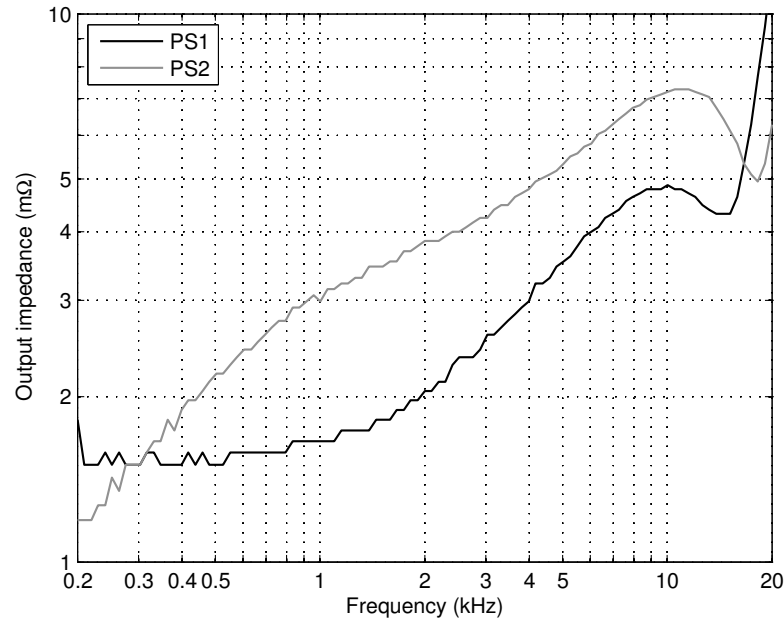
Figure 9.11: Measured output impedance for PS1 and PS2.
