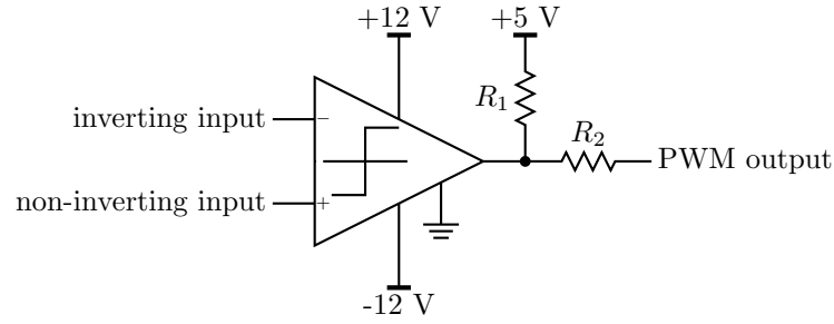
Figure 7.17: The LM306 comparator circuit.
