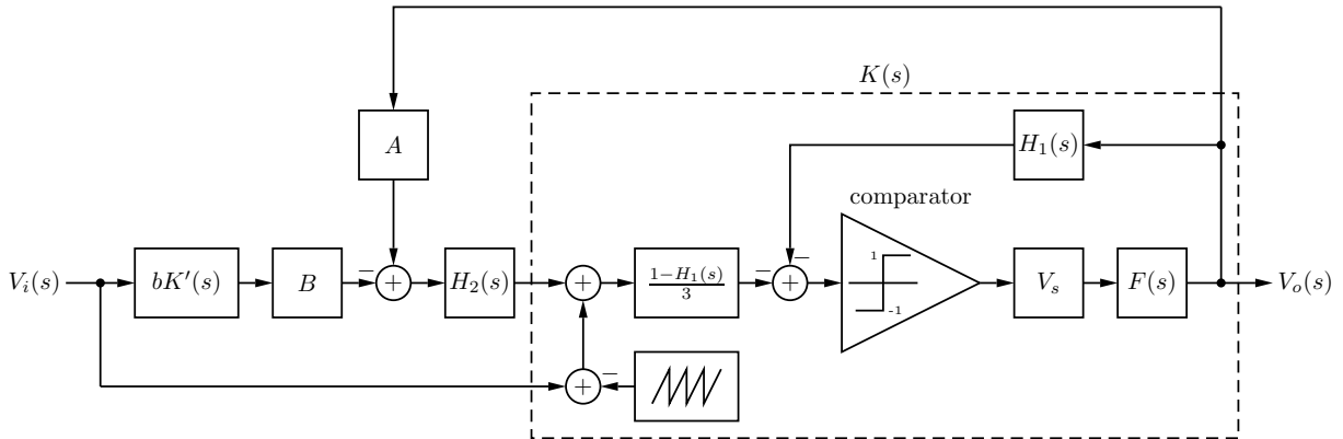
Figure 5.8: Complete control system diagram.
