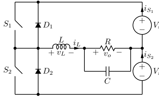
Figure 2.4: Simplified half-bridge converter.
