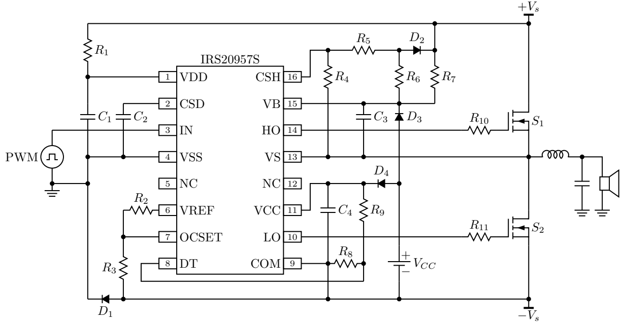
Figure 3.2: IRS20957S gate driver implementation.
