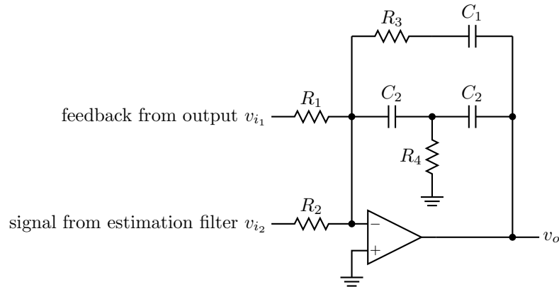
Figure 5.6: Single op-amp third-order integrating loop filter.
