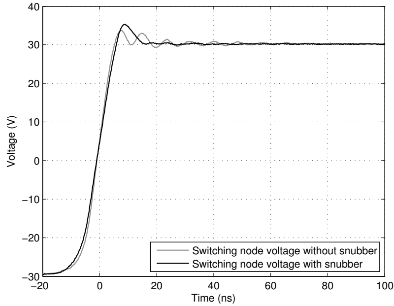
Figure 3.16: Oscilloscope measurement of switching node voltage with and without RC snubber.
