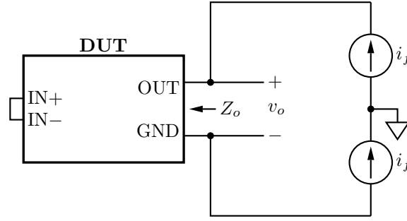
Figure 9.10: Output impedance measurement setup.
