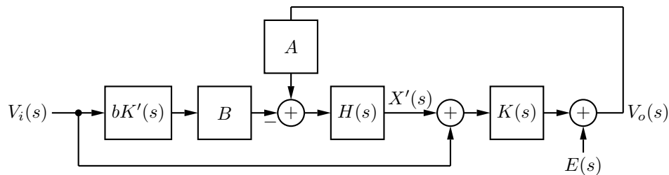
Figure 7.8: General control system with estimation filter.
