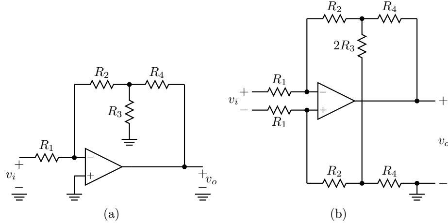
Figure 5.2: Shunt voltage feedback op-amp circuit (a) and its balanced equivalent (b).
