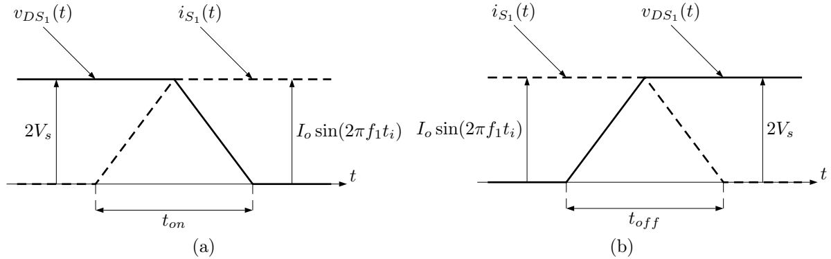
Figure 3.9: Idealised MOSFET switching waveforms during (a) turn-on and (b) turn-off.
