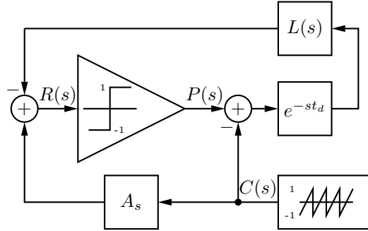
Figure 6.3: Block diagram for comparator gain calculation.
