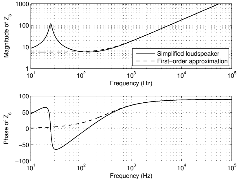
Figure 7.2: Calculated impedance of the simplified loudspeaker and the first-order approximation.
