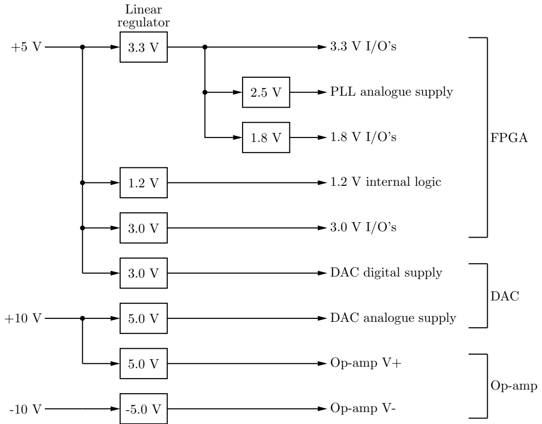
Figure 4.5: Power distribution of the carrier generator board.
