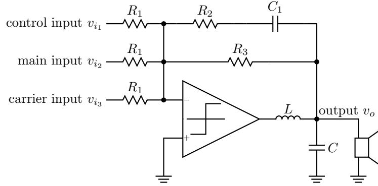
Figure 7.4: Output stage with single pole passive lead compensation.
