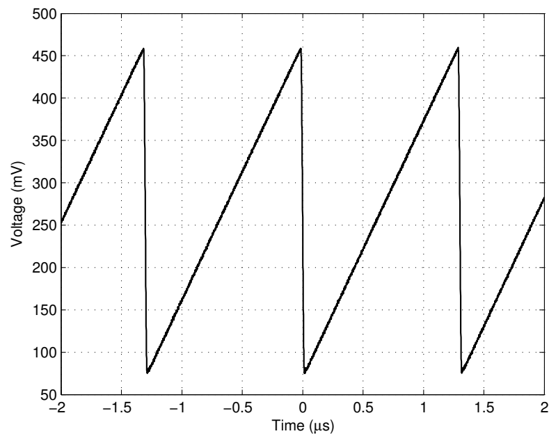
Figure 4.7: Measured carrier generator output at V_{OUT+} for a sawtooth waveform. The Fourier summation is limited to N = 10,000 terms.
