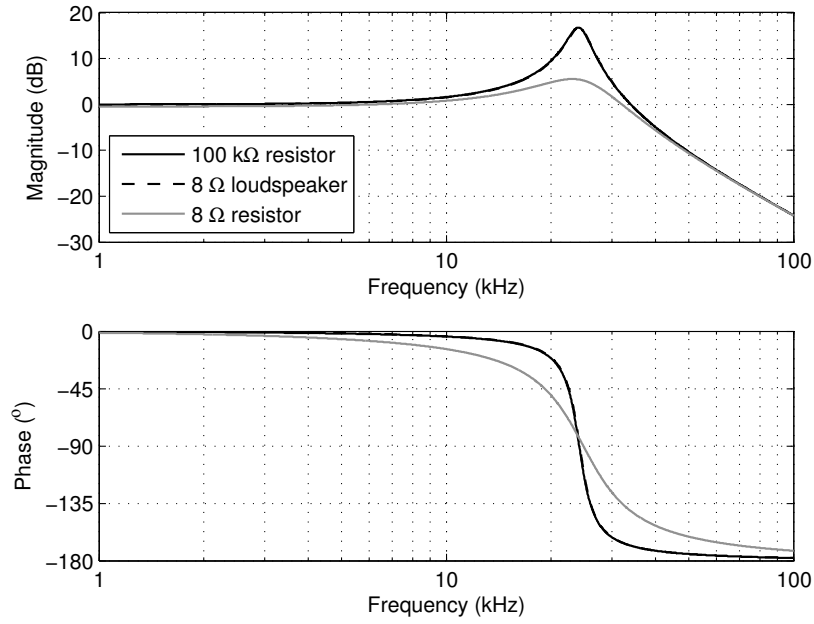
Figure 7.3: Calculated demodulation filter transfer function for a 100 k \Omega resistor, an 8 \Omega loudspeaker, and an 8 \Omega resistor as load, respectively.
