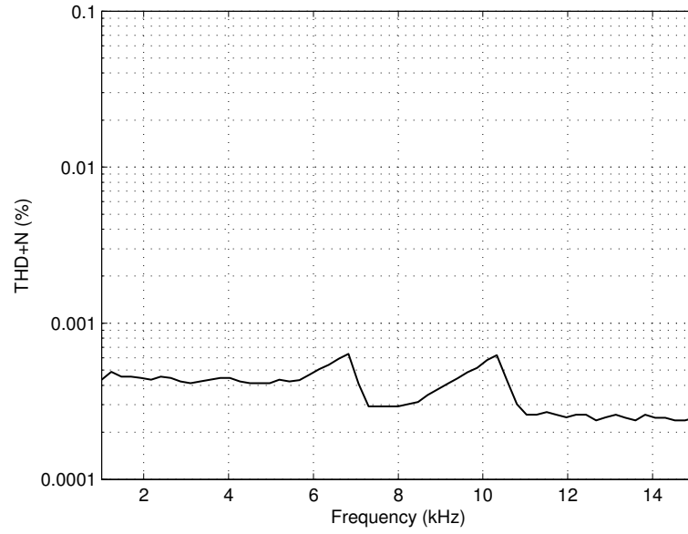
Figure 9.16: Measured THD+N versus frequency of PS1 at 10 W with R_o = 8.2 \Omega and t_d = 125 ns.
