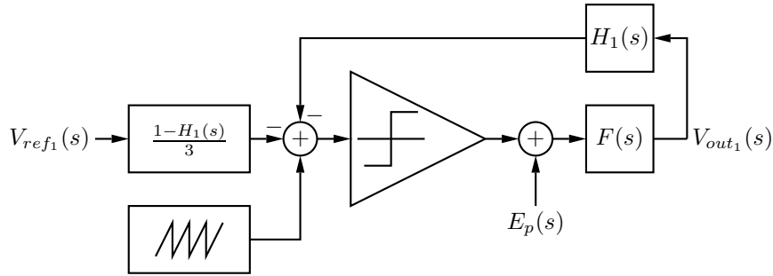
Figure 6.4: Continuous-time inner loop.
