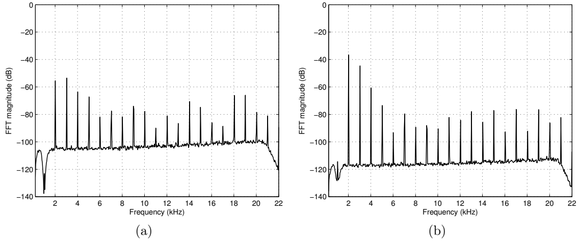
Figure 9.4: FFT of the open loop distortion residue with 10 W at 1 kHz into 8.2 \Omega for (a) PS1 and (b) PS2. THD+N is (a) 0.295% and (b) 1.587%. The suppressed fundamental is at 0 dB.
