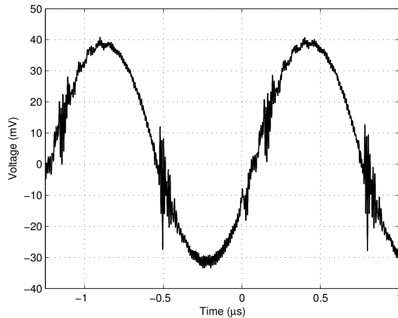
Figure 3.15: Oscilloscope measurement of the amplifier output signal with no input reference signal. Measurement bandwidth is 100 MHz.
