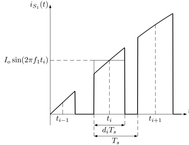
Figure 3.8: Current through MOSFET S_1 with a sinusoidal current source as load. Three switching cycles are shown.
