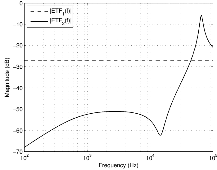
Figure 7.14: Calculated magnitude versus frequency of ETF_1(f) and ETF_2(f) for an 8.2 \Omega load.
