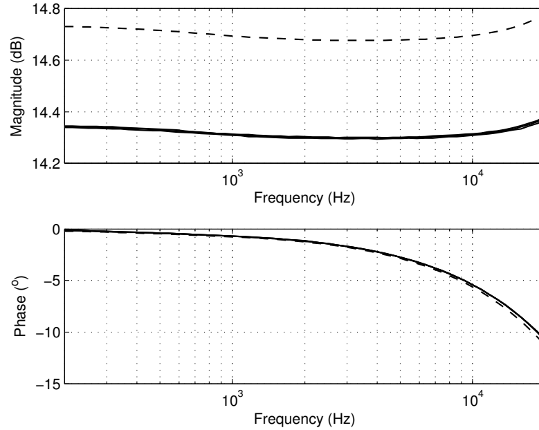
Figure 9.9: Measured closed loop frequency response of the complete control loop for various output loads. From top to bottom: R_o = 100 \text{ k}\Omega , R_o = 8.2 \text{ }\Omega and R_o = 4.1 \text{ }\Omega . The dashed line is the theoretical frequency response for an 8.2 \text{ }\Omega load.
