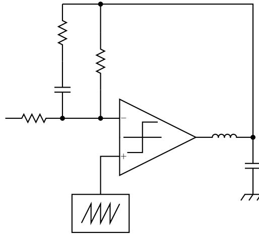
Figure 2.15: Output stage with passive lead network.
