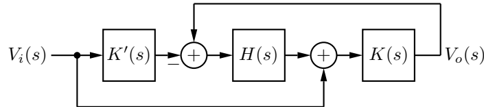
Figure 5.1: Basic control loop structure.
