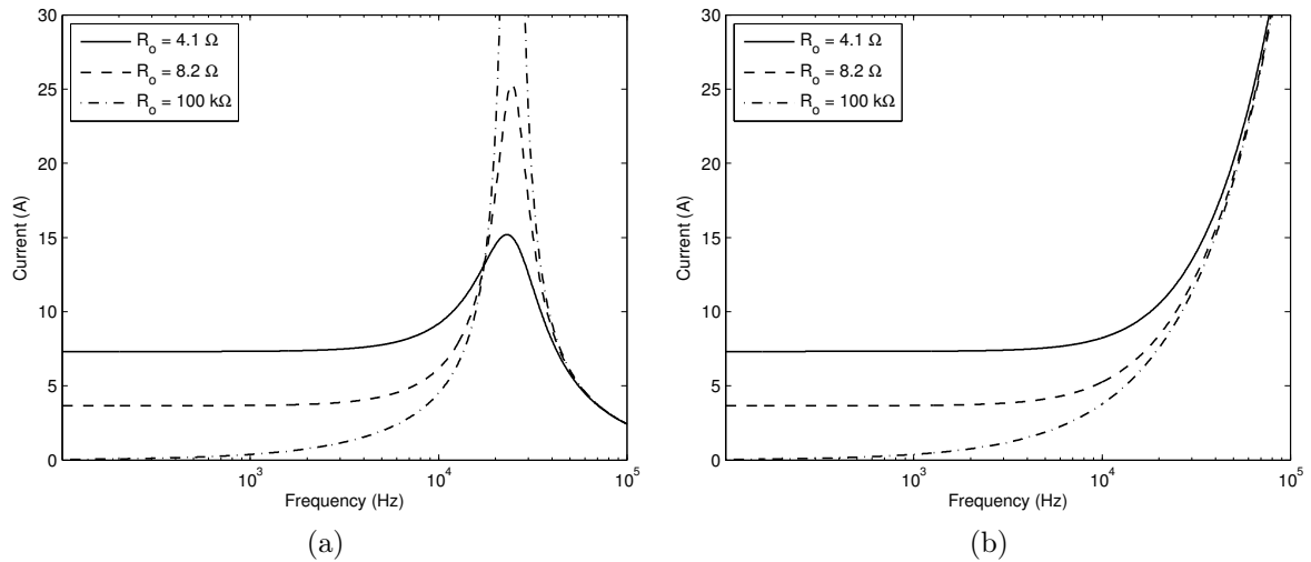
Figure 3.14: Calculated demodulation filter input current for an output voltage of 30 V at 1 kHz for (a) the open loop converter and (b) the closed loop converter.
