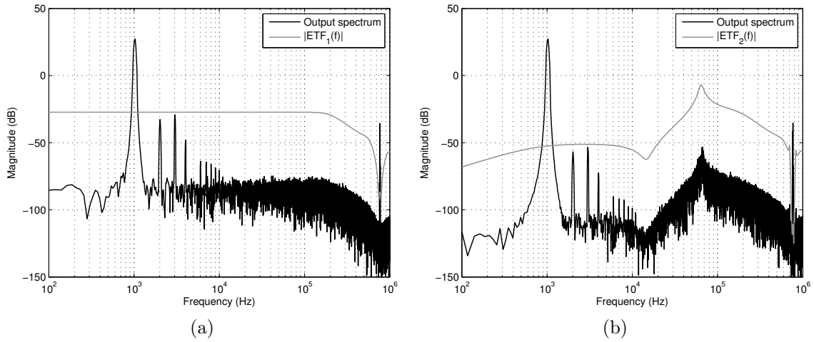
Figure 8.2: Magnitude spectrum of simulated amplifier output without ripple compensation with only the inner loop active (a) and with both loops active (b). The error transfer functions are shown in grey for comparison.
