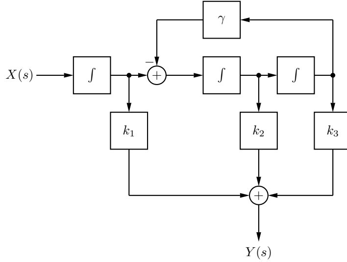
Figure 5.5: Third-order integrating loop filter with local feedback and feed-forward summation.
