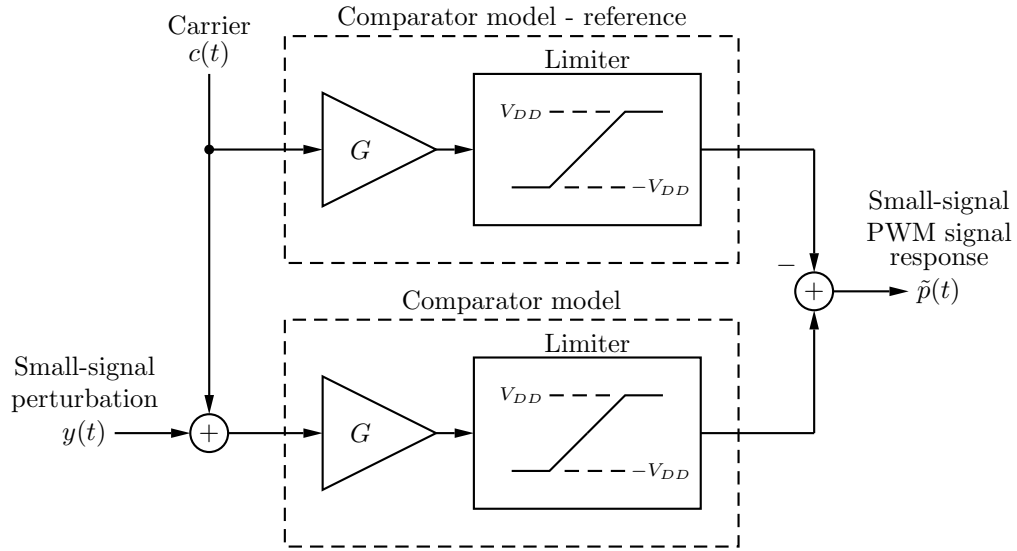
Figure 2.6: Small-signal comparator model [1].
