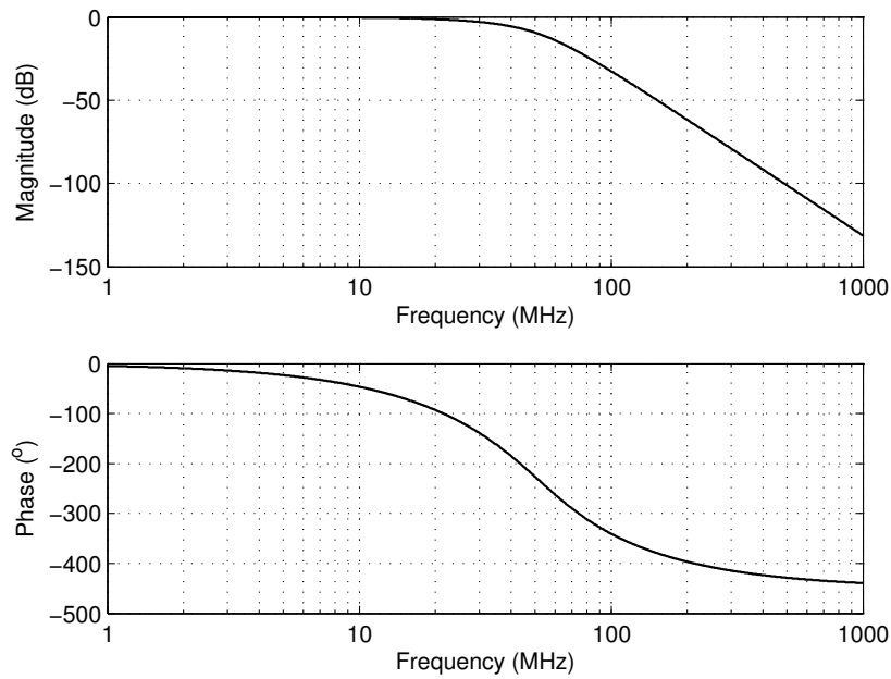
Figure 4.4: Frequency response of the DAC output filter.
