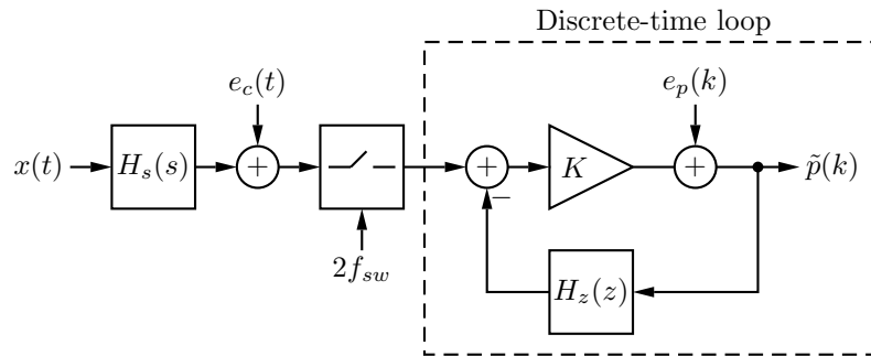
Figure 2.9: Discrete-time comparator model embedded in a feedback loop.
