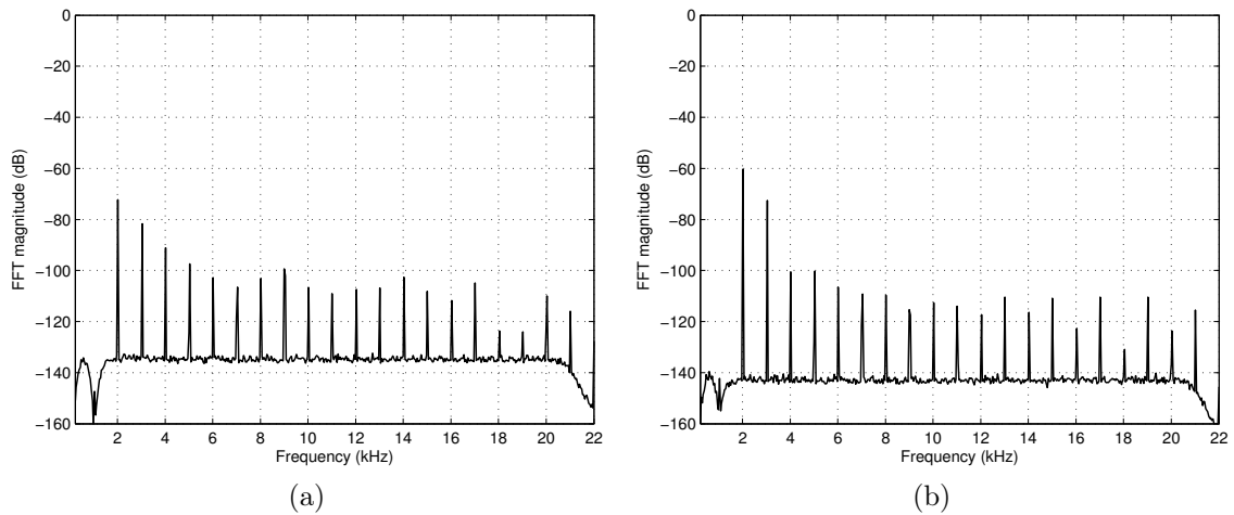
Figure 9.5: FFT of the distortion residue with the inner loop active with 10 W at 1 kHz into 8.2 \Omega for (a) PS1 and (b) PS2. THD+N is (a) 0.0254% and (b) 0.0985%. The suppressed fundamental is at 0 dB.
