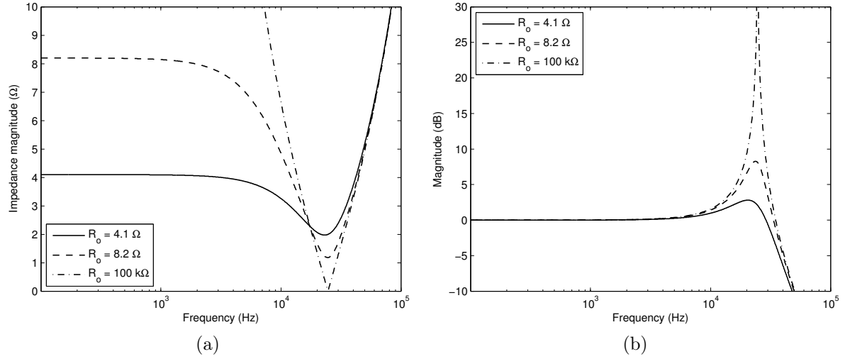
Figure 3.13: (a) Calculated input impedance of the demodulation filter. (b) Calculated magnitude response of the demodulation filter.
