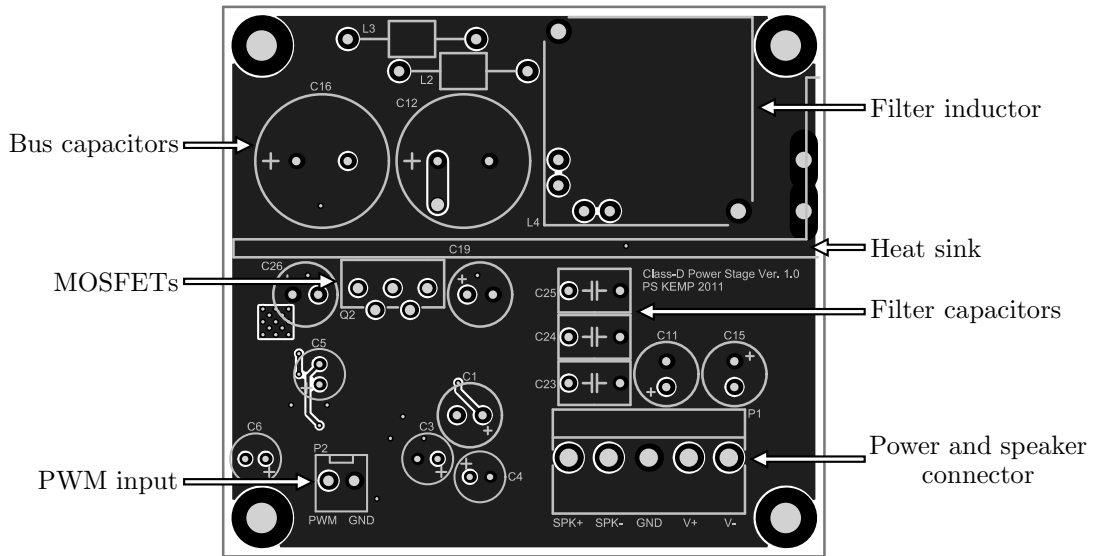
Figure 3.11: Top layer of PCB.
