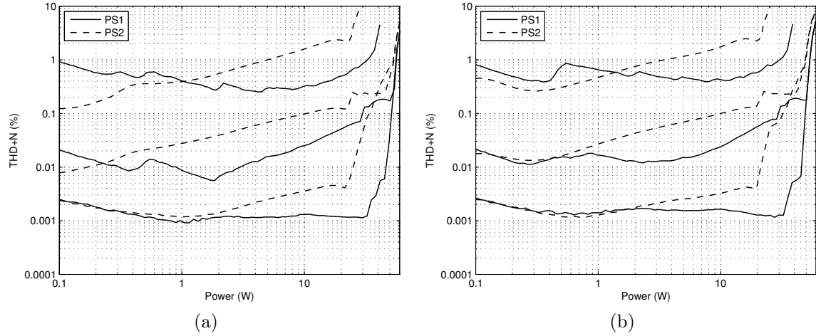
Figure 9.2: Measured THD+N versus output power at 1 kHz with (a) R_o = 8.2 \Omega and (b) R_o = 4.1 \Omega . From top to bottom: open loop, with the inner control loop active, and with the complete control loop active.
