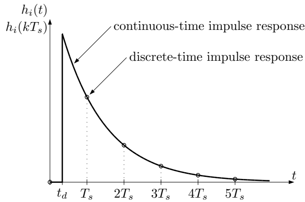
Figure 6.2: Continuous-time and discrete-time impulse responses.
