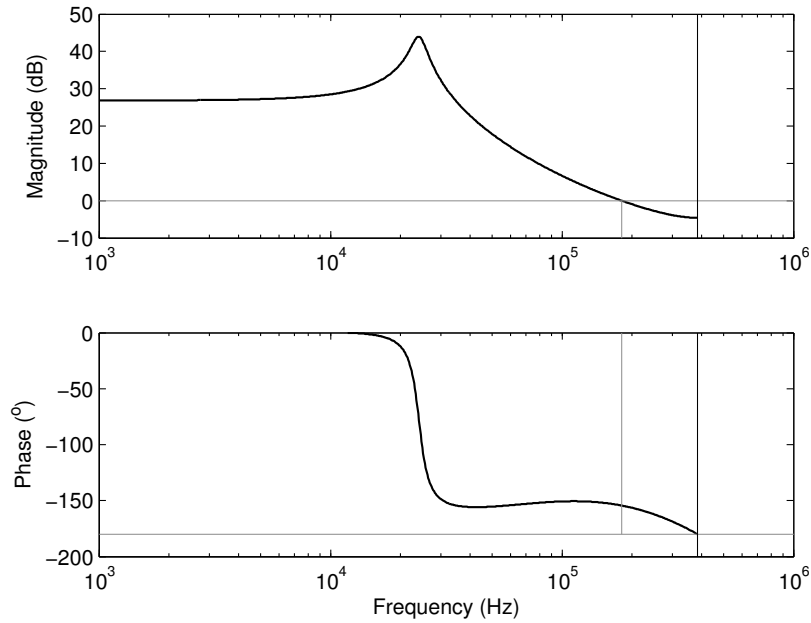
Figure 7.11: Bode plot of KG_1(z) for a 100 \text{ k}\Omega load and a propagation delay of t_d = 150 \text{ ns} . Gain margin is 4.59 \text{ dB} and phase margin is 25.6^\circ .
