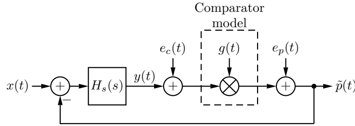
Figure 2.8: Comparator model embedded in a feedback loop.
