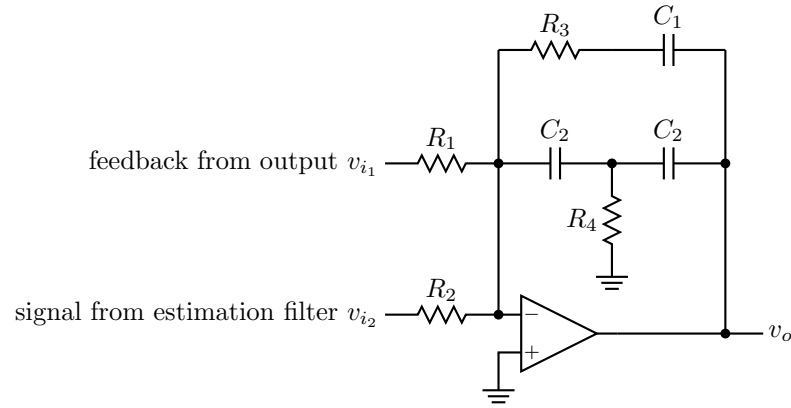
Figure 7.5: Single op-amp third-order integrating loop filter.
