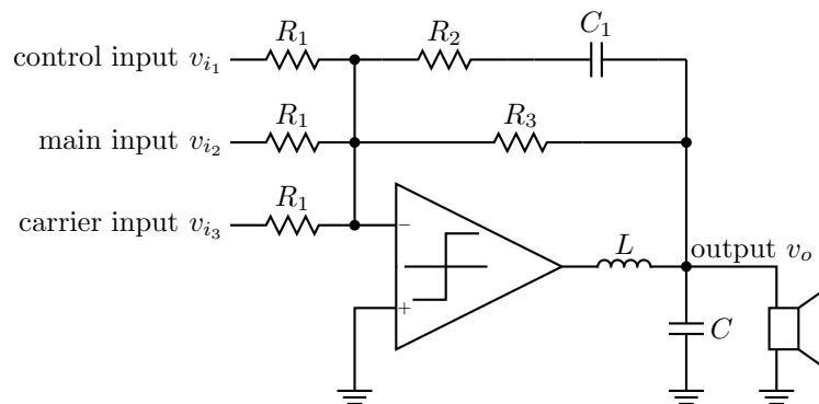
Figure 5.3: Output stage with passive lead compensation.
