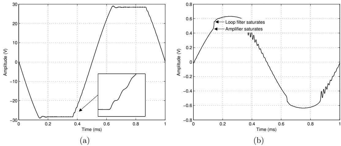
Figure 8.5: Spice simulation of amplifier output (a) and outer loop filter output (b) during over-modulation for R_2 = 3.3 \text{ k}\Omega .
