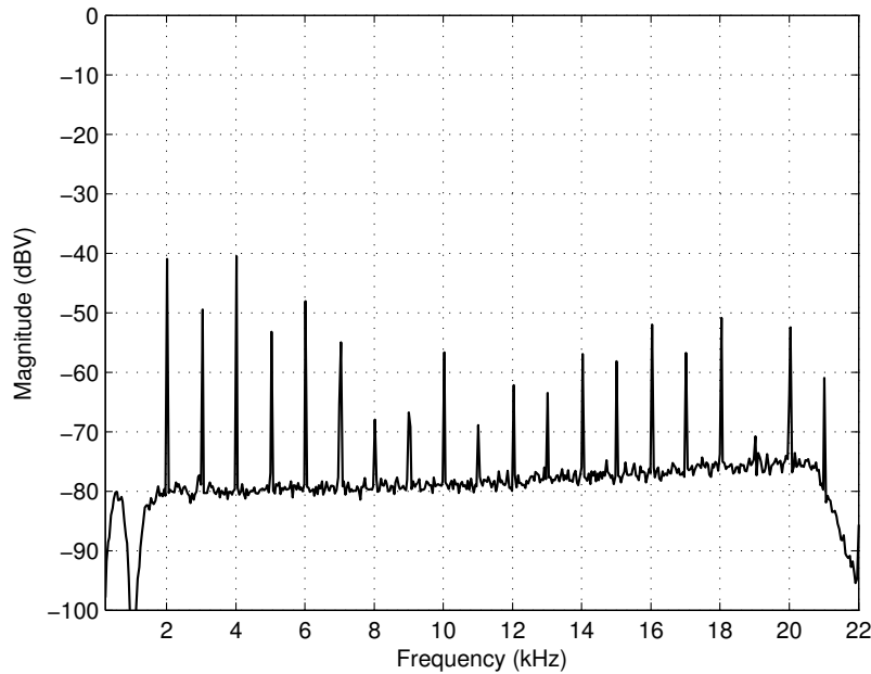
Figure 3.18: FFT of distortion residue with 100 mW into 8.2 \Omega . The suppressed fundamental is at 0 dBV.
