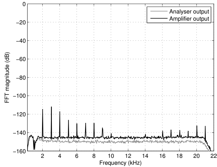
Figure 9.17: FFT of the distortion residue of PS1 with 10 W at 1 kHz into 8.2 \Omega for t_d = 125 ns. THD+N is 0.00044%. The suppressed fundamental is at 0 dB.
