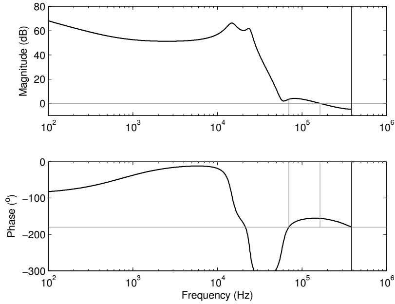
Figure 7.12: Bode plot of K[G_1(z) + G_2(z)] for a 100 k \Omega load and a propagation delay of t_d = 150 ns. Gain margin is -3.43 dB and phase margin is 23.9^\circ .
