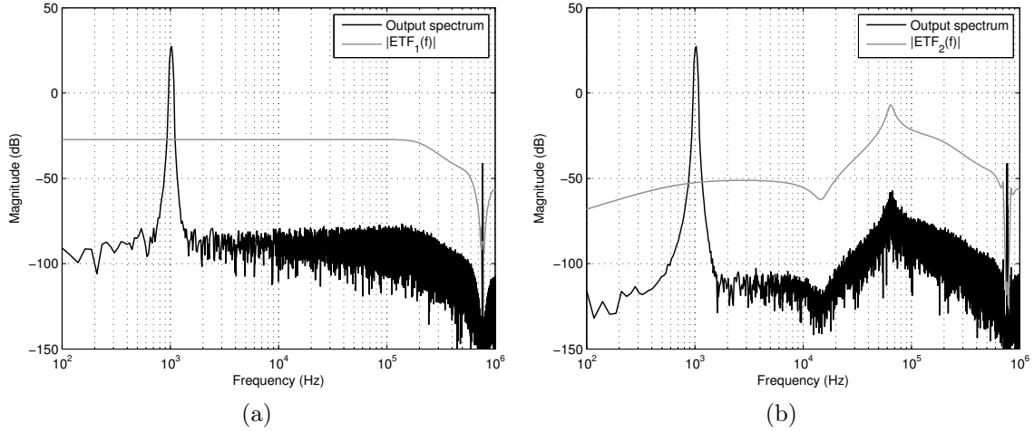
Figure 8.1: Magnitude spectrum of simulated amplifier output with only the inner loop active (a) and with both loops active (b). The error transfer functions are shown in grey for comparison.
