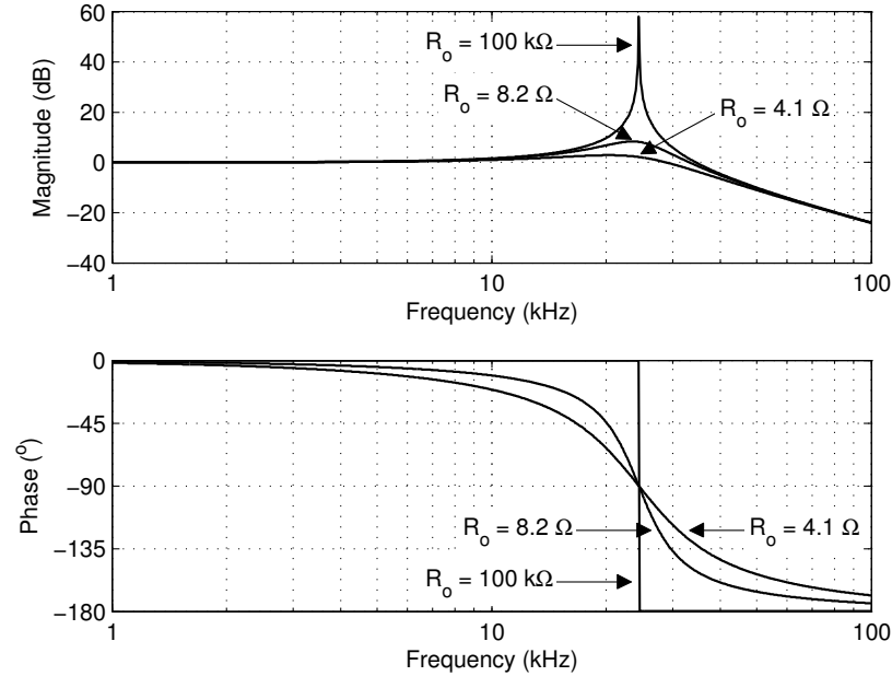
Figure 3.10: Calculated frequency response of the ideal demodulation filter for various output loads.
