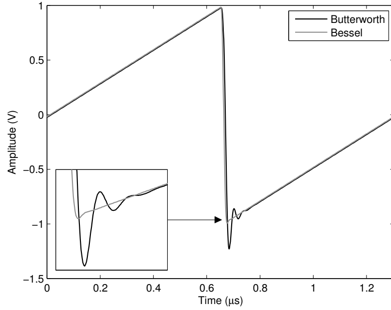
Figure 4.3: Filtered sawtooth signal for a 5th order Bessel and Butterworth filter.
