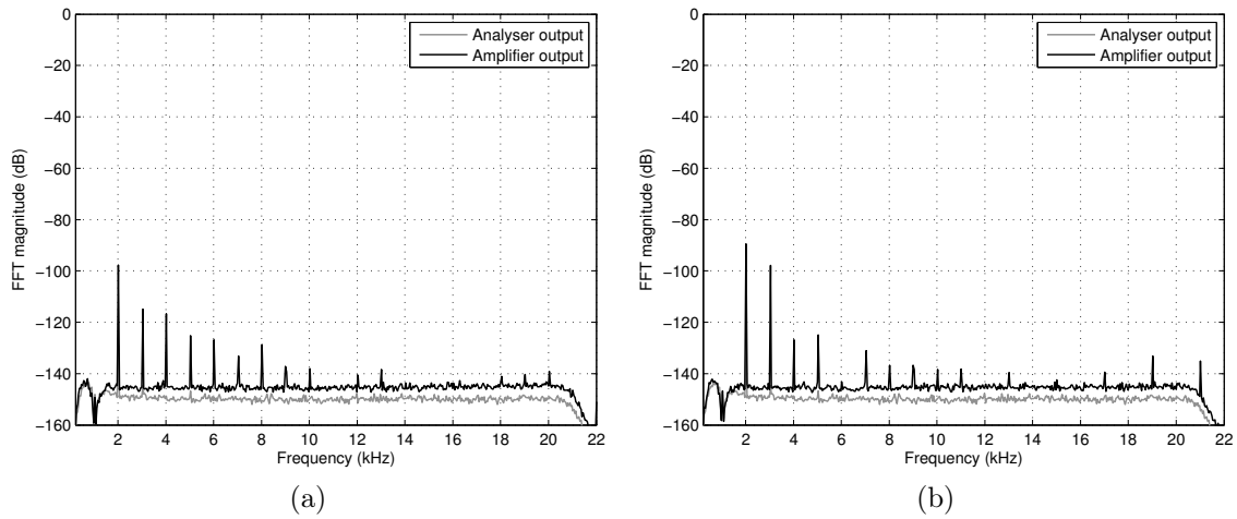
Figure 9.6: FFT of the distortion residue with both loops active with 10 W at 1 kHz into 8.2 \Omega for (a) PS1 and (b) PS2. THD+N is (a) 0.00132% and (b) 0.00354%. The suppressed fundamental is at 0 dB.
