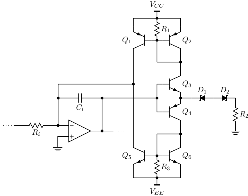
Figure 2.16: Transistor-based loop filter saturation circuit.
