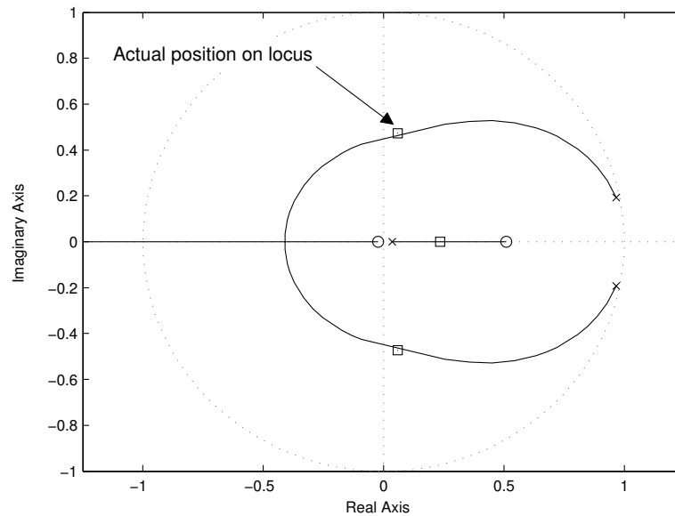
Figure 7.9: Root locus of the inner control loop with an output load of R_o = 100 \text{ k}\Omega .
