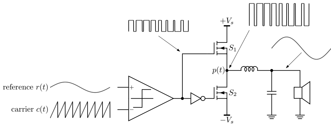
Figure 1.1: Basic class-D operation.
