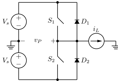
Figure 2.2: Simplified half-bridge inverter with current-source load.
