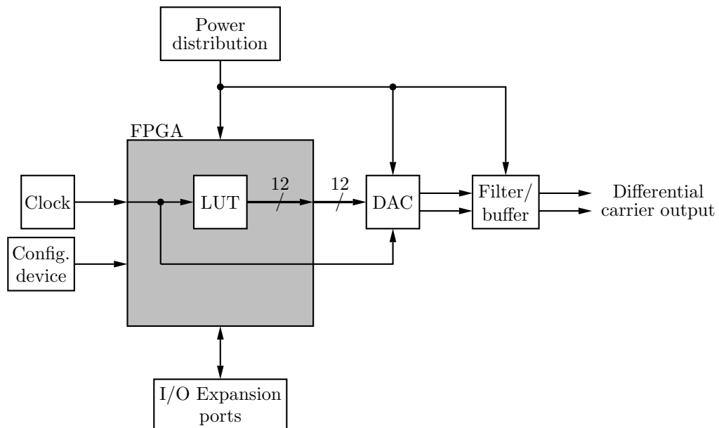
Figure 4.1: Block-diagram of the FPGA-based carrier generator.
