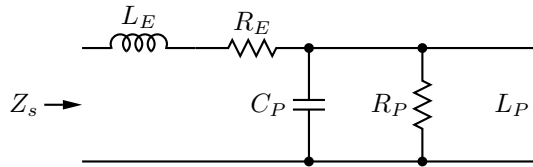
Figure 7.1: Simplified equivalent circuit of a moving-coil transducer.
