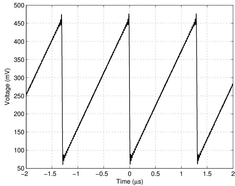
Figure 4.6: Measured carrier generator output at V_{OUT+} for a sawtooth waveform. The Fourier summation is limited to N = 63 terms.
