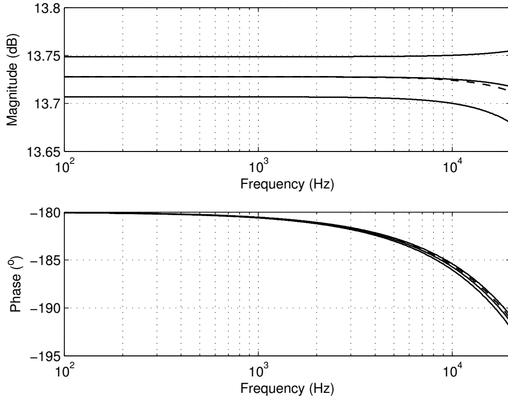
Figure 7.7: Calculated closed-loop transfer function STF_1(f) of the inner loop for various output loads R_o . From top to bottom: R_o = 100 \text{ k}\Omega , R_o = 8.2 \text{ }\Omega and R_o = 4.1 \text{ }\Omega . The dotted line is the transfer function K'(f) of the estimation filter.
