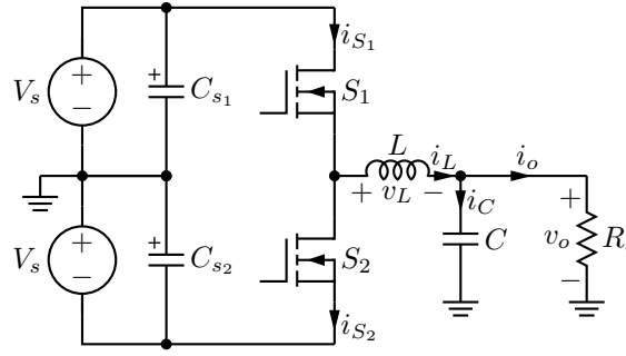
Figure 3.1: Half-bridge topology.
