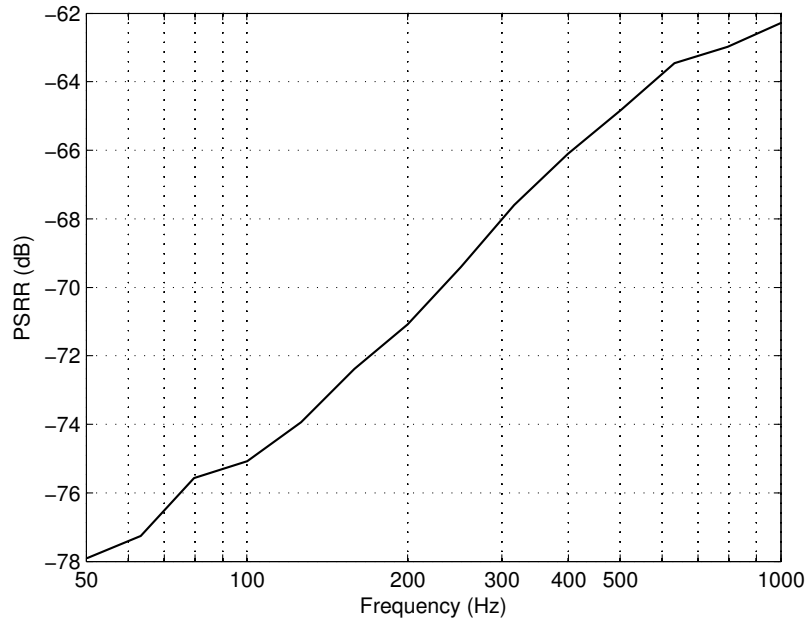
Figure 9.13: Measured PSRR as a function of frequency.
