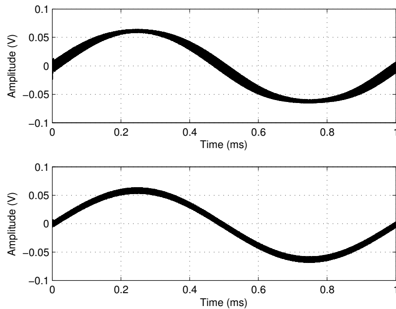
Figure 8.4: Simulated comparator input reference signal without ripple compensation (top) and with ripple compensation (bottom). The input signal frequency is 1 kHz and m_a = 0.8 .
