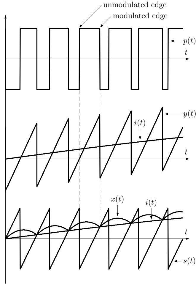
Figure 2.11: Ripple compensation waveforms for a first-order loop [2].
