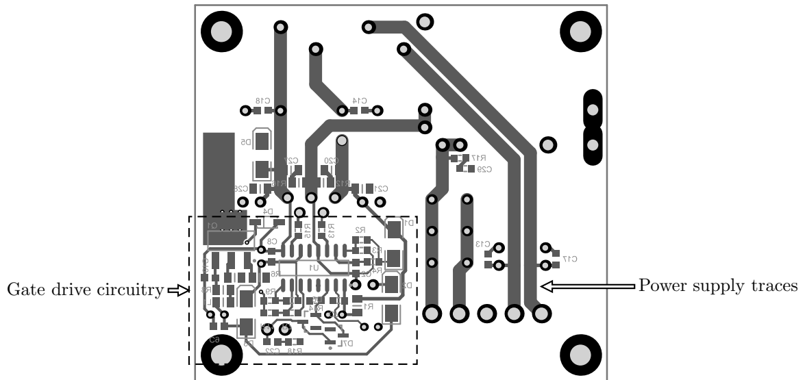
Figure 3.12: Bottom layer of PCB.
