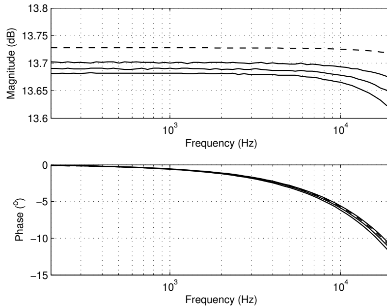
Figure 9.8: Measured closed loop frequency response of the inner loop for various output loads. From top to bottom: R_o = 100 \text{ k}\Omega , R_o = 8.2 \text{ }\Omega and R_o = 4.1 \text{ }\Omega . The dashed line is the theoretical frequency response for an 8.2 \Omega load.
