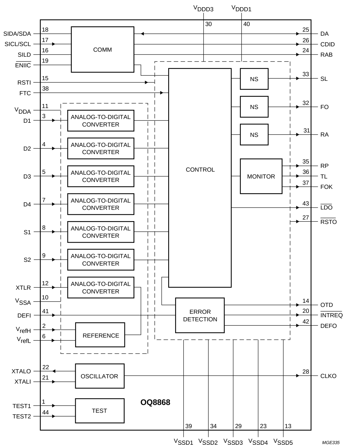
Fig.1 Block diagram.
