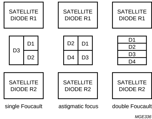
Fig.3 Detector arrangement.
