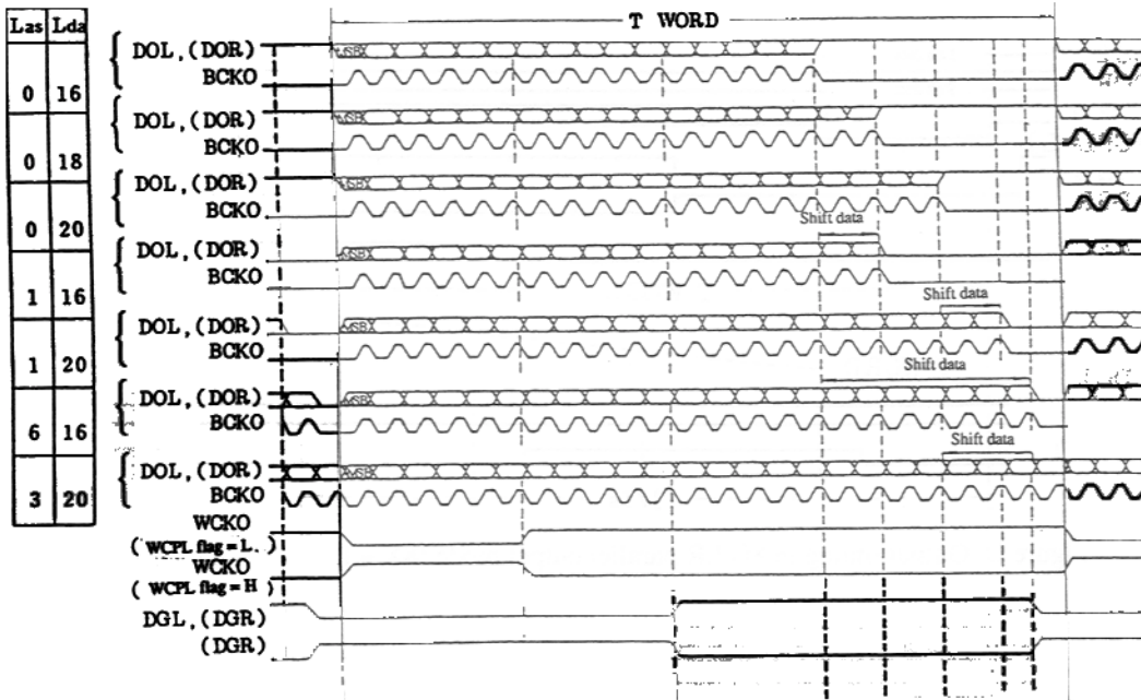
Figure B Unit output word timing (when CKSL = H)
