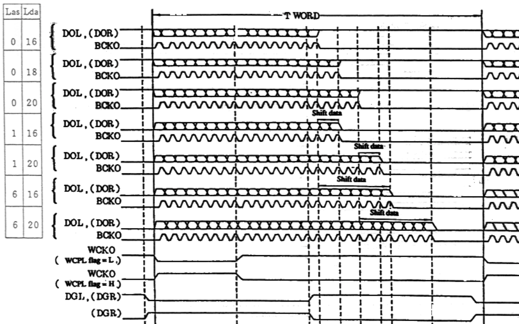
Figure C Unit output word timing (when CKSL = L)
