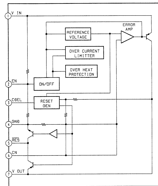
IC201 LA5602
