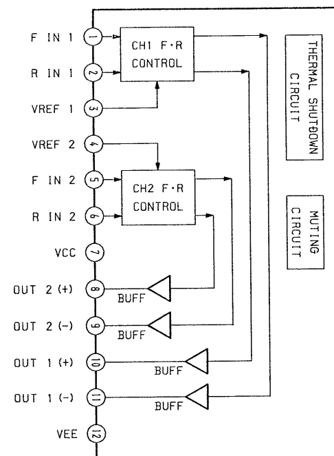
IC451 BA6191
