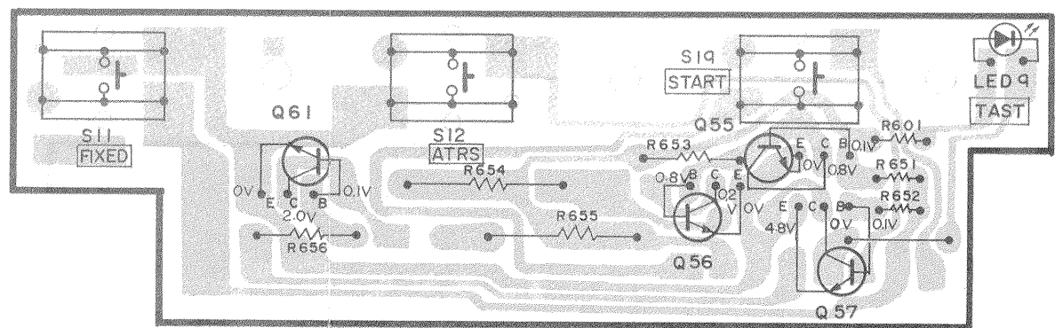
ATRS PC Board
