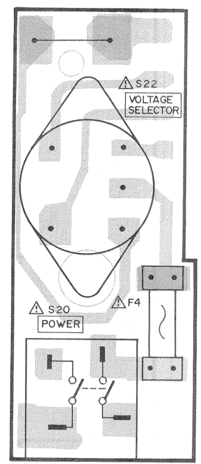
Power PC Board (For W)
