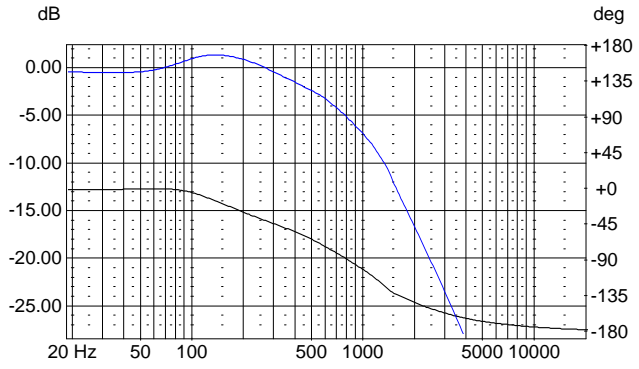
Net 2 gain
