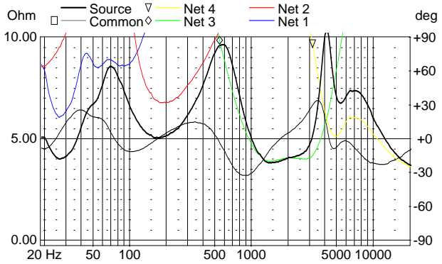
Input impedance
