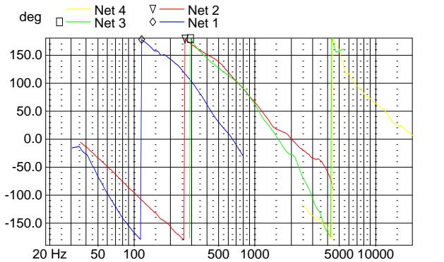
Individual phase response
