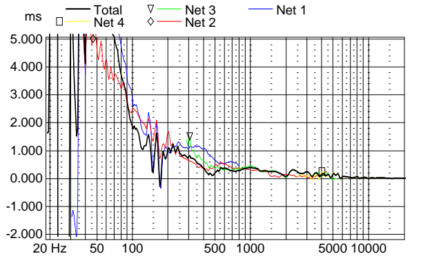
Group delay
