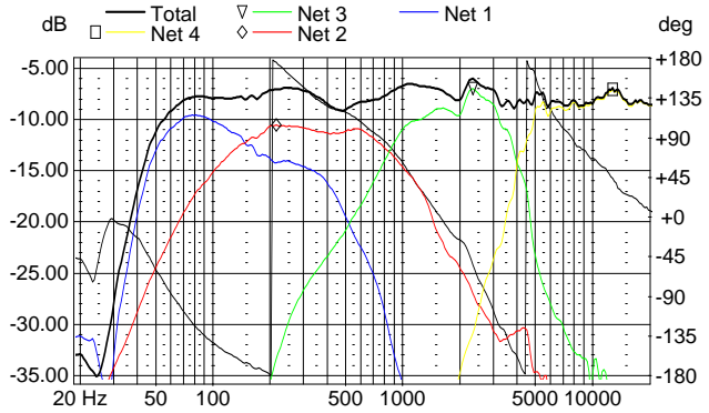
Summed frequency response
