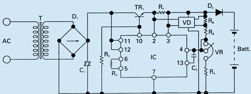
Figure 21. EXAMPLE OF A TWO STAGE CONSTANT VOLTAGE, CURRENT LIMITED CHARGING CIRCUIT
