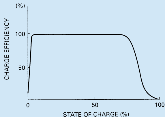
Figure 30. CHARGING EFFICIENCY VS STATE OF CHARGE
