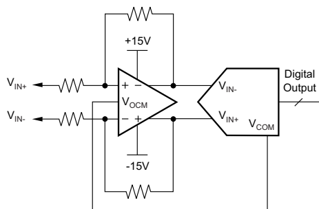
Typical ADC Circuit
